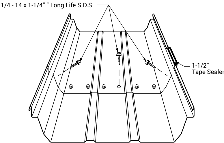
FASTENER SEQUENCE FIRST RUN - ENDLAP
