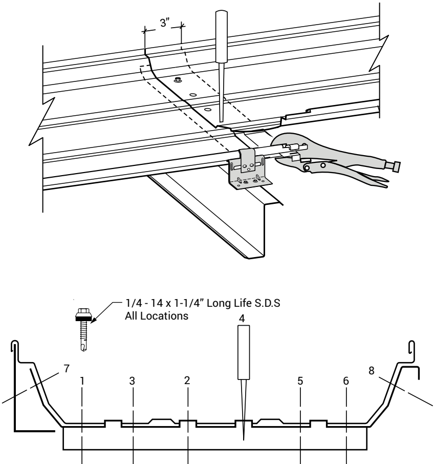
FASTENER SEQUENCE FIRST RUN - ENDLAP
