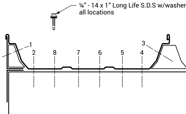
FASTENER SEQUENCE FIRST RUN - EAVE
