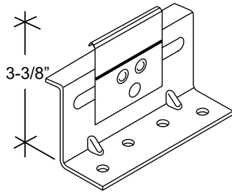
HW-2102 - 2" LOW SLIDING CLIP
